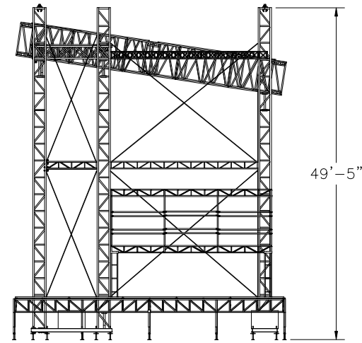
Stage Left Elevation
